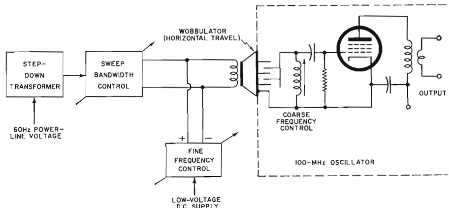
Fig. 5. A 100-MHz oscillator with wobbulator frequency control.
