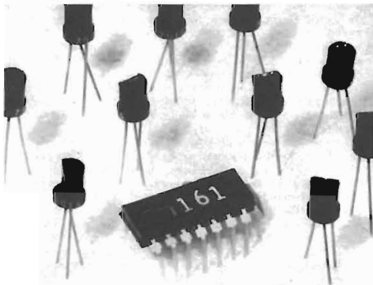
Fig. 4. A flat plastic package with 7 leads on each side and an extra heat-sink lead is used to house the IC. The highly mechanized production line that turns out these packages is an outgrowth of work on plastic-packaged silicon transistors shown.
