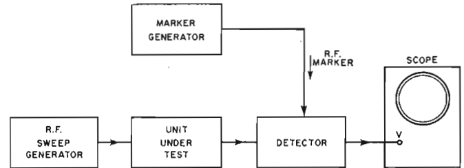
Fig. 10. Simple marker-injection system is illustrated here.
