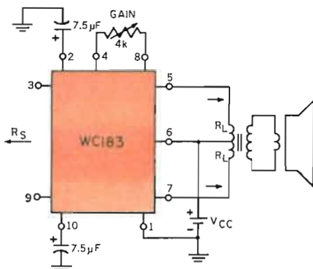
R_S —TYPICAL 5000 \Omega A.C. AND 600 \Omega D.C. R_L —TYPICAL 250 \Omega A.C. AT 1kHz
