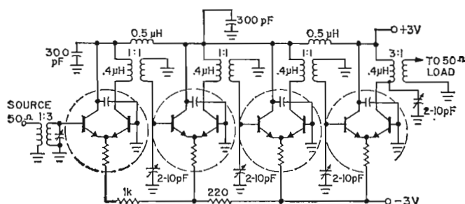
Fig. 4. A 60-MHz radar i.f. amplifier using four MC1110 IC's.
