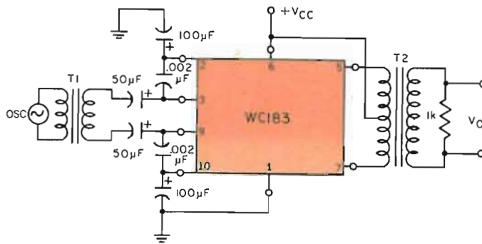
TRANSFORMERS: T1—GENERAL RADIO TYPE 941-A OR EQUIV. T2—PEERLESS TYPE E-204-D OR EQUIV.
