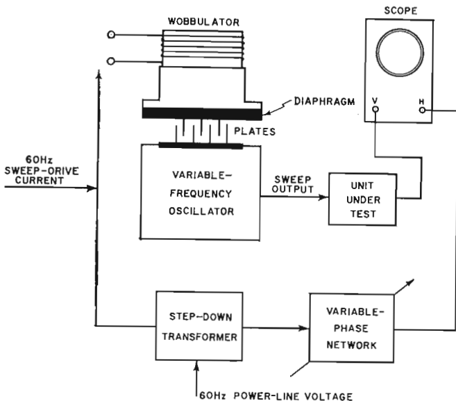
Fig. 3. Principle of the wobbulator-driven sweep generator.
