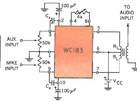
R_L —TYPICAL 250 \Omega A.C. C_e —EQUALIZATION CAPACITOR
