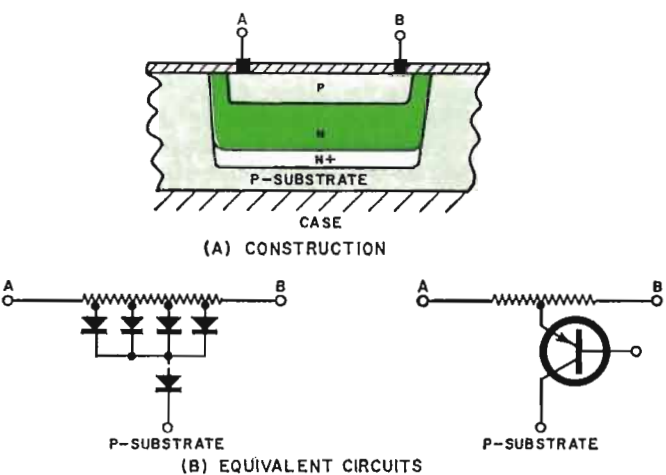
Fig. 4. Construction and equivalent circuit of IC resistor
