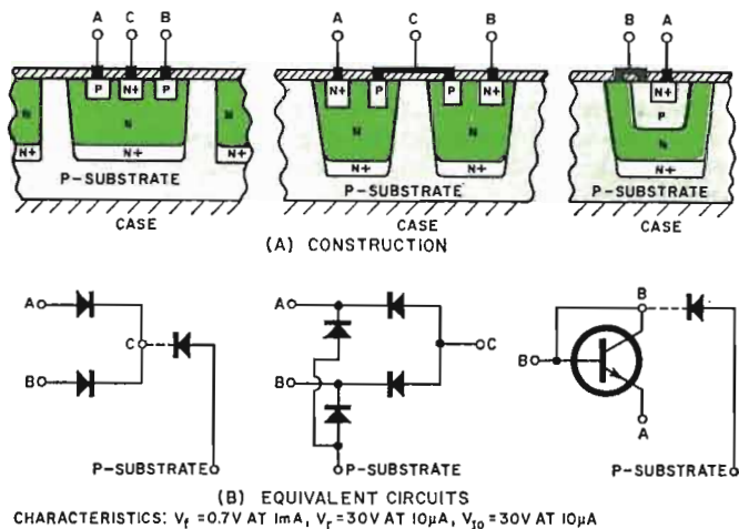
Fig. 3. Silicon monolithic integrated-circuit diodes.
