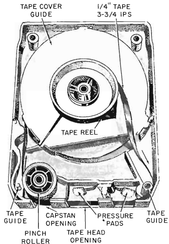
Fig. 2. The Lear cartridge also consists of a single reel of specially lubricated tape in a continuous loop. The operation is similar to the Fidelipac except that a pinch roller is built into the cartridge itself and this is engaged by tape capstan.
