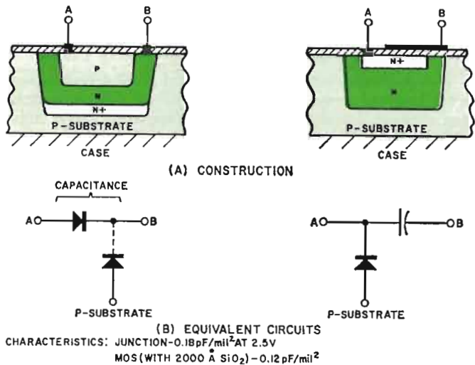
Fig. 6. Equivalent circuits, characteristics of IC capacitors.
