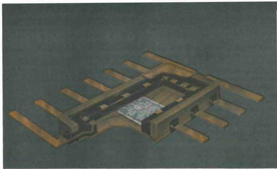
Cutaway view of integrated circuit mounted in 14-lead flat pack.
