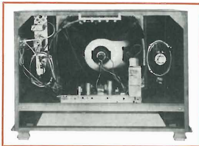
Fig. 1. The Magnavox T908 chassis can drive a 24-inch CRT.
