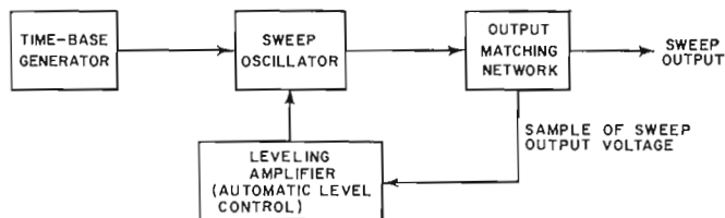
Fig. 1. Block diagram of basic sweep frequency generator.
