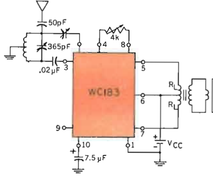
R_L —TYPICAL 250 \Omega A.C. AT 1kHz
