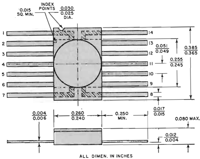
Fig. 8. The 14-lead flat package, along with its dimensions.
