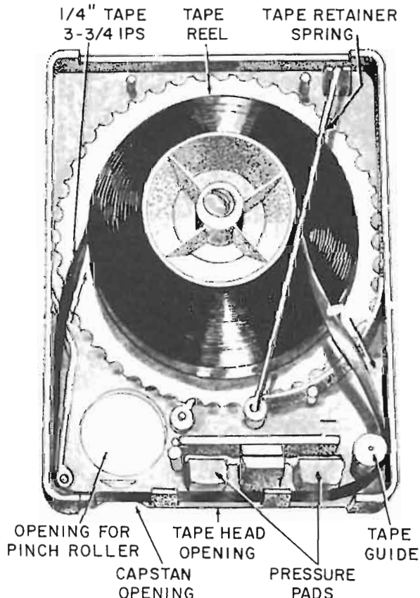
Fig. 1. The Fidelipac (TelePro) cartridge consists of a single reel of specially lubricated tape arranged as a continuous loop. The tape comes off the center of the reel and moves around the tape guide and past the two pressure pads and tape head. It then goes between pinch roller and capstan which are on the tape deck and engage the tape through openings in cartridge. The tape then returns to the outside of the tape reel, completing the loop.
