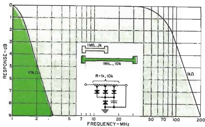
Fig. 5. Frequency characteristics of pair of IC resistors.
